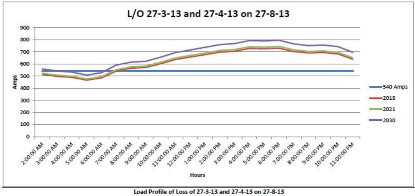
Figure 1. Peak Day Load profile for circuit 27-8-13 for the simultaneous loss of circuits 27-3-13 and 27-4-13
