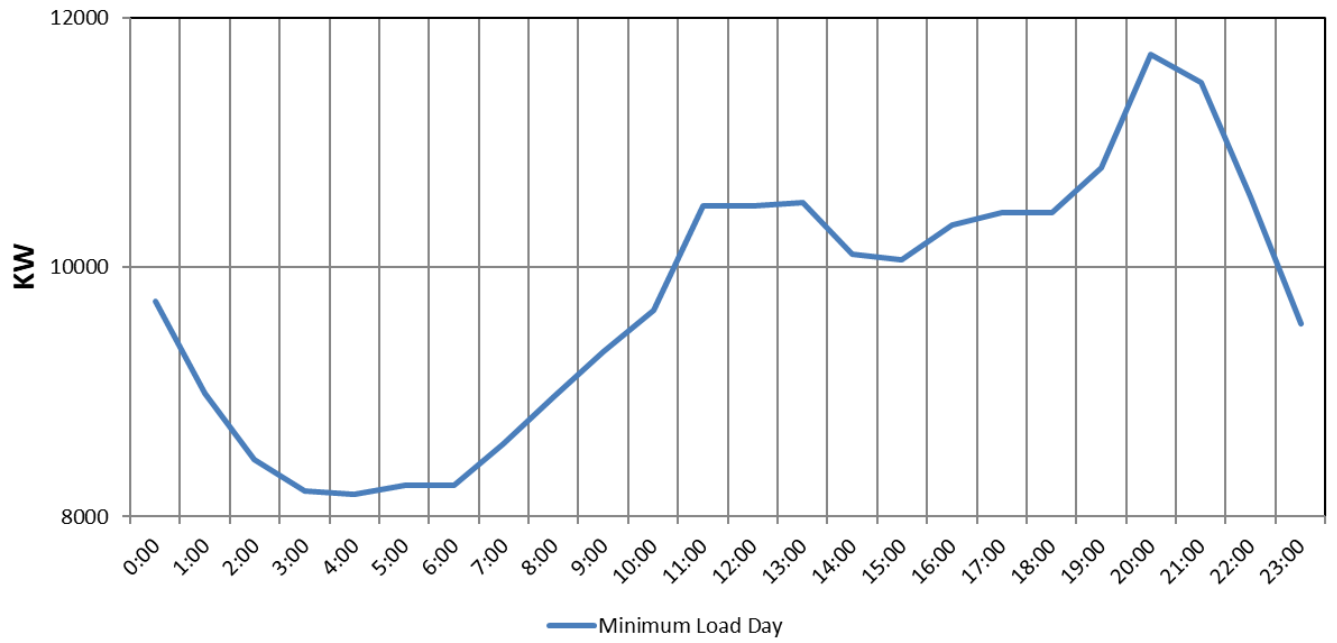
Nyack Area Station #2 - Minimum 2019 Load Day
