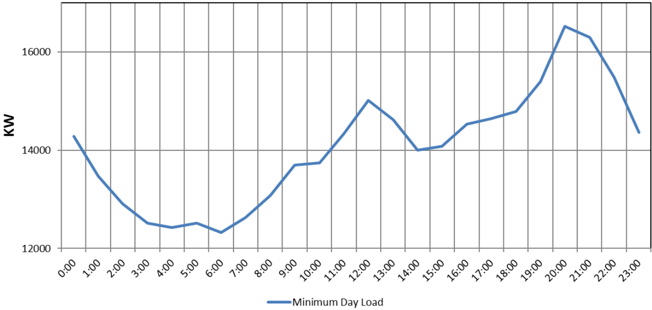
Haverstraw Area Station - Minimum 2019 Load Day
